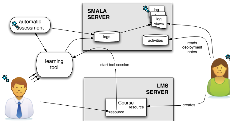
Figure 8-6: System architecture corresponding to the SMALA model.
